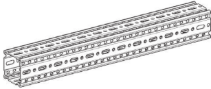
Single-span beam with uniaxial load dead weight of the profile is considered
