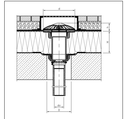
Warmdach, begehbar (Terrasse), Massivdach, SDA-Speed, PK-NG Rohr
